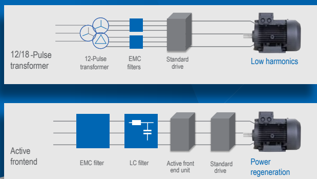
Conventional low harmonics and regenerative solutions
