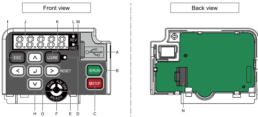
Figure 1.1 Keypad
