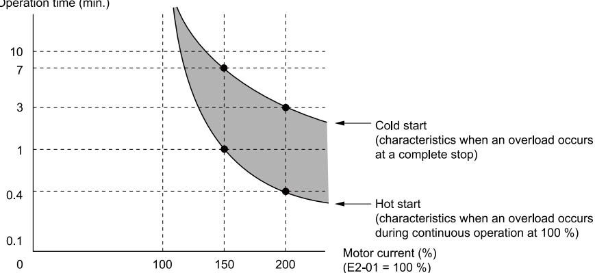
Figure 10.6 Protection Operation Time for a General-purpose Motor at Rated Output Frequency
